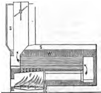
FIG. 59.—Stevens's Return Tubular Boiler, 1832.
